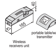
Wireless receivers unit portable table/wall transmitter
