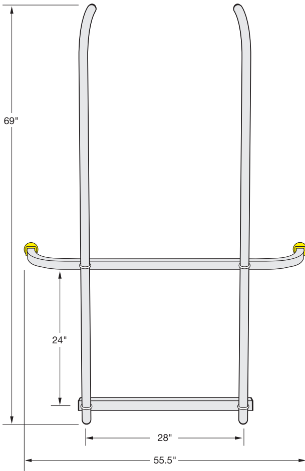
Fully Extended Dimensions
