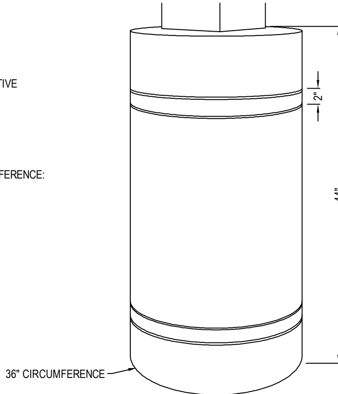
PERSPECTIVE
