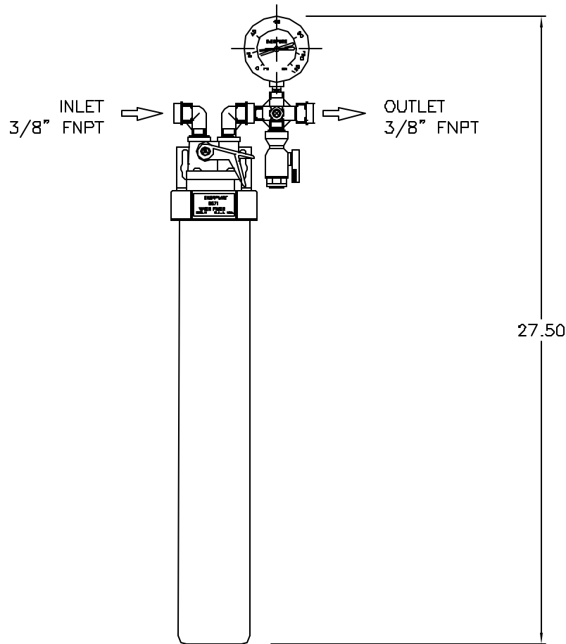
FRONT VIEW
