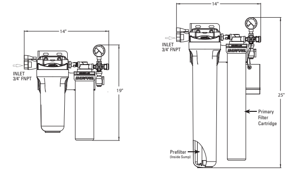
Figure 5 – Insurice PF Single 4FC-S & 7FC-S System(s)
