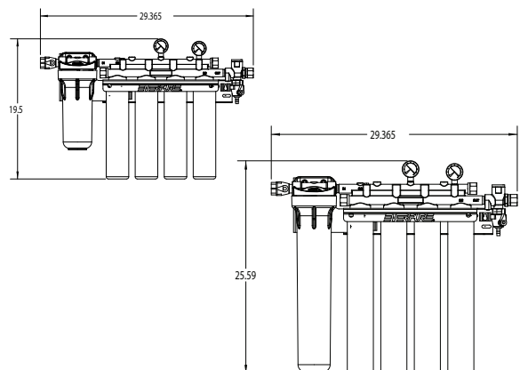
Figure 8 - Insurice PF Quad 4FC-S & 7FC-S System(s)
