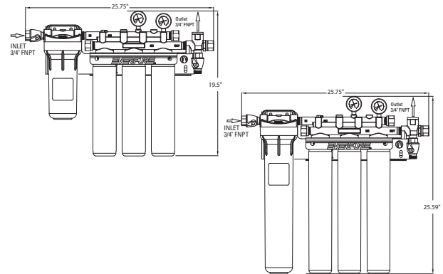
Figure 7 – Insurice PF Triple 4FC-S & 7FC-S System(s)
