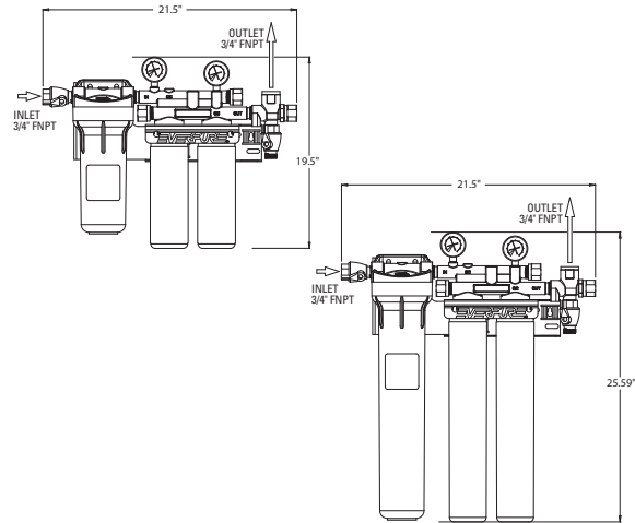
Figure 6 – Insurice PF Twin 4FC-S & 7FC-S System(s)
