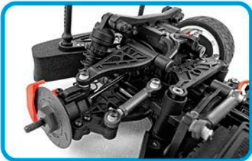
For better handling, A-arm front and rear independent suspension keeps the Hoonitruck under control during the wildest of driving conditions
