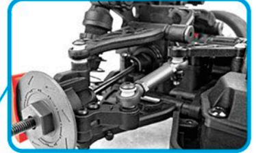
Active rear suspension allows the amount of toe change to be adjusted through the suspension cycle, increasing or decreasing rear grip
