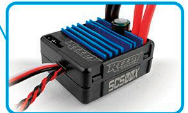
Reedy SC500X programmable brushed ESC (program card sold separately)
