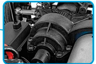
A sealed center driveline keeps dirt and debris out--along with bits of tire rubber--for smooth and reliable power delivery
