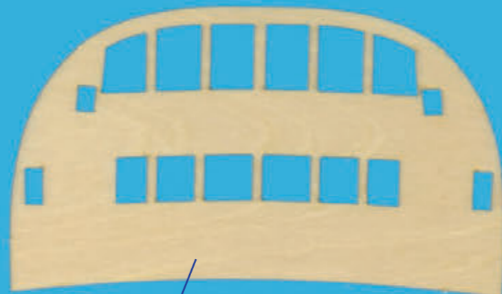
34 2 mm plywood PRE 1 pc
