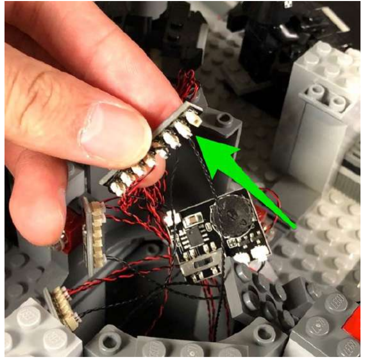
23.) Tuck the 6-port expansion board and cabling in behind the stair case and left pillar as shown below
