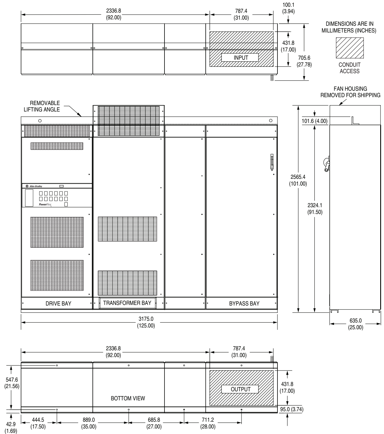
Figure 31. PowerFlex 700H 18 Pulse, Frame 11, NEMA/UL Type 1 - with Bypass
