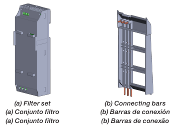
Figure A1: (a) and (b) Parts of the CFW300-KFA filter kit Figure A1: (a) e (b) Peças do kit filtro CFW300-KFA
