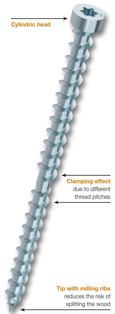
HECO-TOPIX®-CombiConnect
