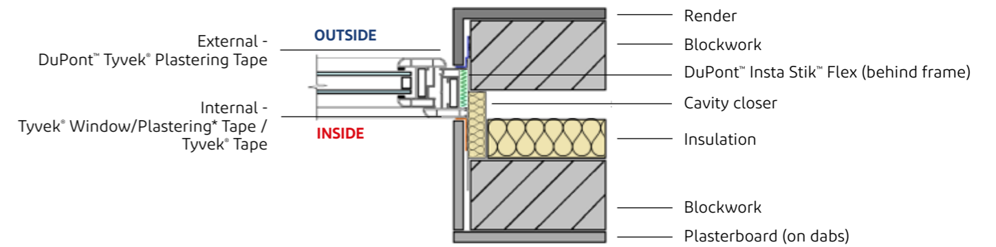
Fig. 1 - Blockwork cavity wall
