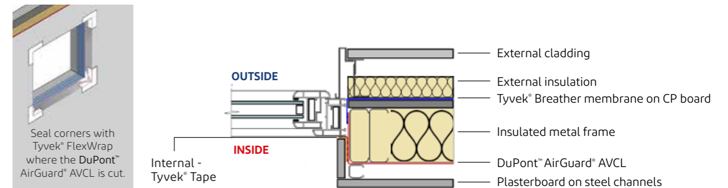
Fig. 2 - SFS aluminium rainscreen
