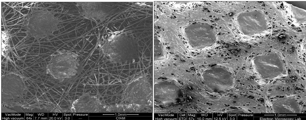
Figure 1. Surface of a thermal bonded PP spunbond fabric in a BRM (64x magnification).
