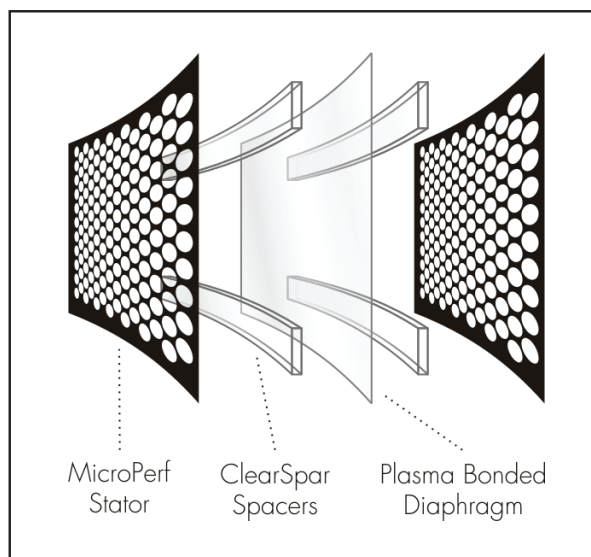
Figure 16. Cut away view of an electrostatic transducer. Notice the simplicity due to minimal parts usage.
