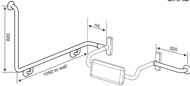
▲ BT36 + RE05R + RE00/300 Available in RH + LH RH shown
