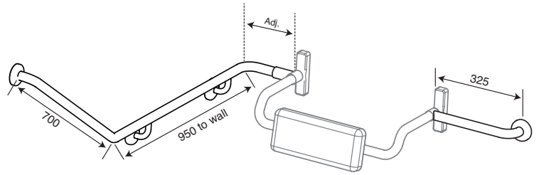
▲ BT36 + RE06R + RE00/300 Available in RH + LH RH shown
