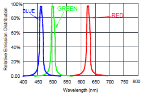
Wavelength Characteristics
