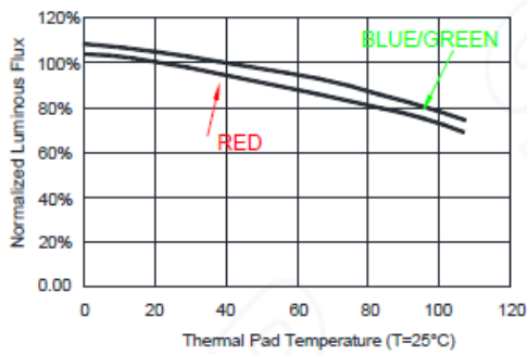
Thermal Pad Temperature vs. Relative Light Output
