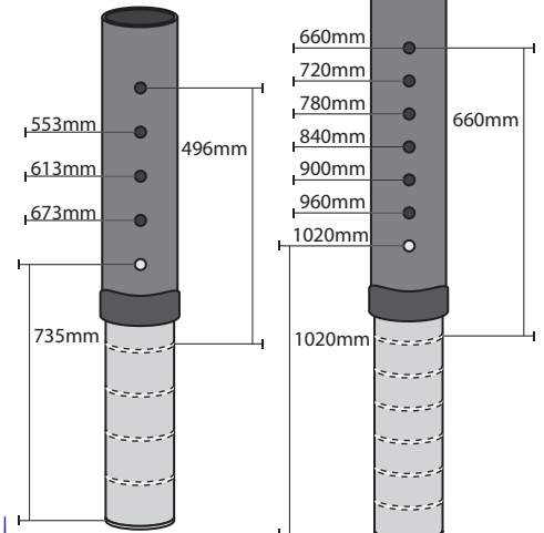
Code 42 Outer: 42mm Dia x 1.6mm RHS Inner: 38mm Dia x 1.6mm RHS Table Height 496 to 735Hmm Counter Height 660mm to 1020mm
