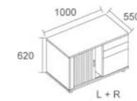
Combination Pedestal (White melamine only)
