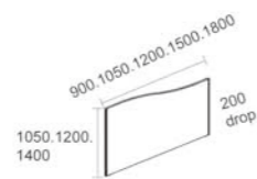
Slimline wave top
