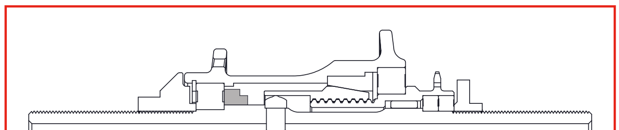
180° SLACK Use Reversed Hat Washer + 0 Tuning Spacers
