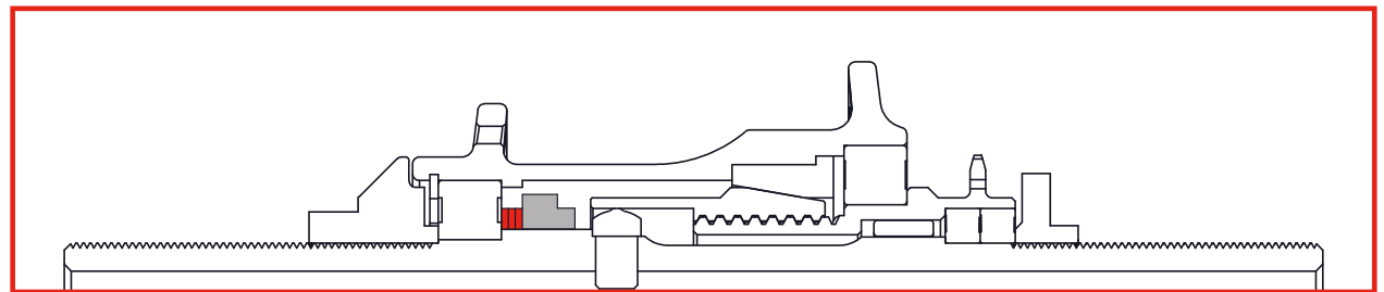
108° SLACK Use Reversed Hat Washer + 3 Tuning Spacers
