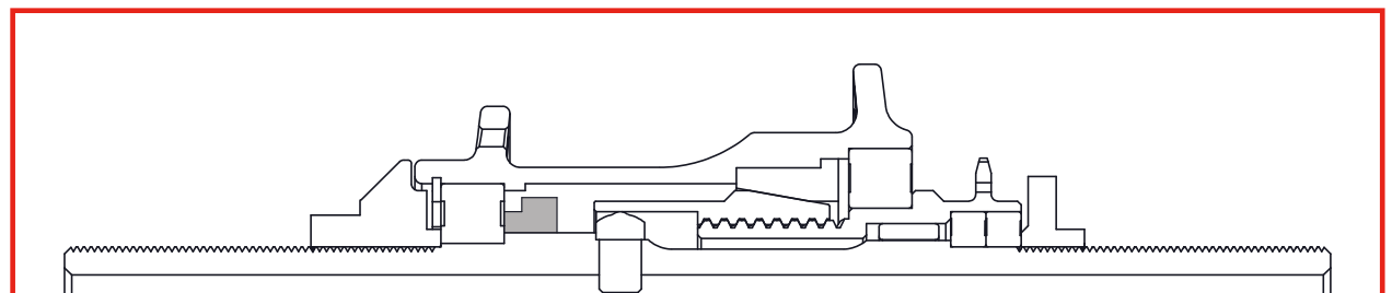
127° SLACK (STANDARD) Use Hat Washer + 0 Tuning Spacers
