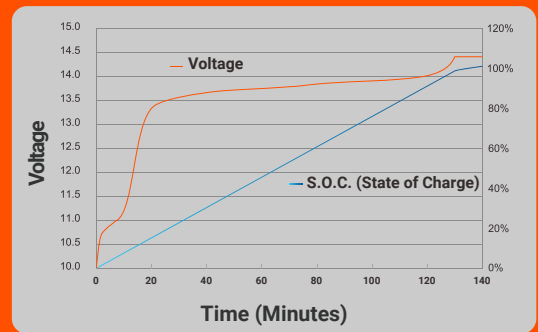
Charge Characteristics (0.5C @ 25°C)
