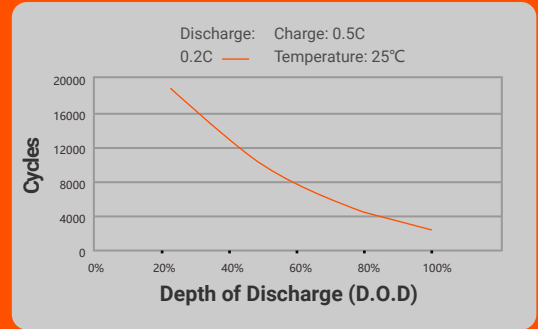
Cycle Life v D.O.D
