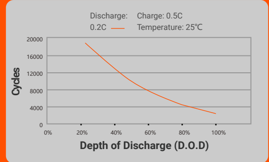
Cycle Life v D.O.D
