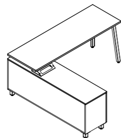
Private Cabin with Return Worktop (*Storage Below Return Worktop)
