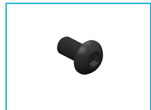
QTY. 3- M5 x 0.8 x 10mm button head screw (Not Included. This is a standard rotor bolt length and can be found at any authorized Felt retailer or bike shop. Note that the 10mm length version MUST only be used, as any other length will result in frame damage.)
