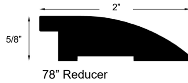
78" Reducer
