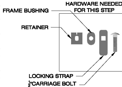
ROTATE THE LOCKING STRAP CLOCKWISE UNTIL IT HITS THE BOTTOM OF THE TRUCK FRAME
