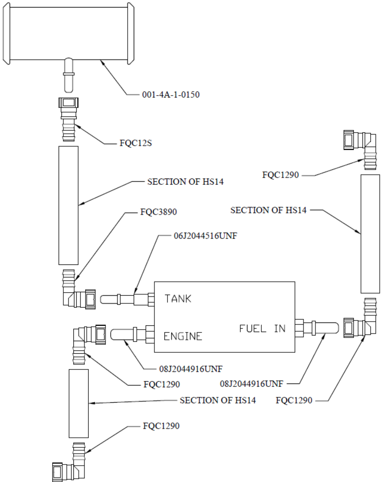
INSIDE FRAME RAIL MOUNTING
