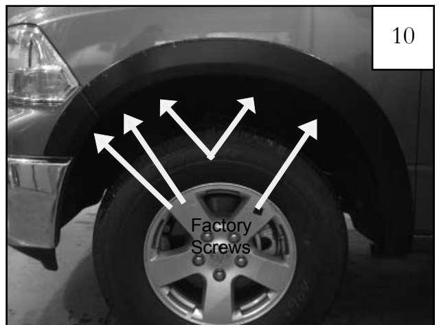
Install supplied screws at indicated locations. See steps 12 & 13.
