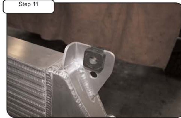
Remove the two upper-rubber isolators with spacers from stock intercooler and install to new BladeRunner® intercooler.
