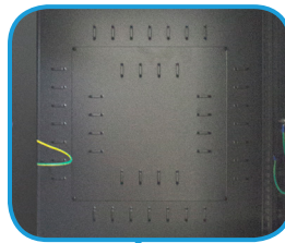
Removable 12" x 12" rear panel for in-wall cable entry
