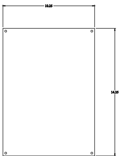
INNER PANEL
