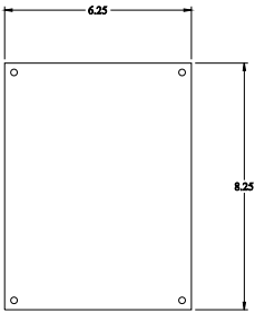
INNER PANEL
