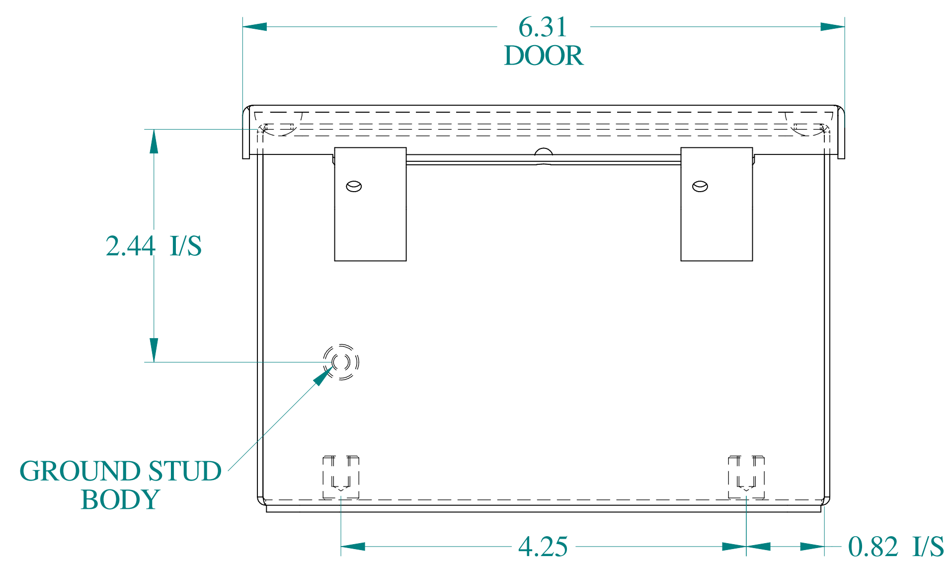
BOTTOM VIEW
