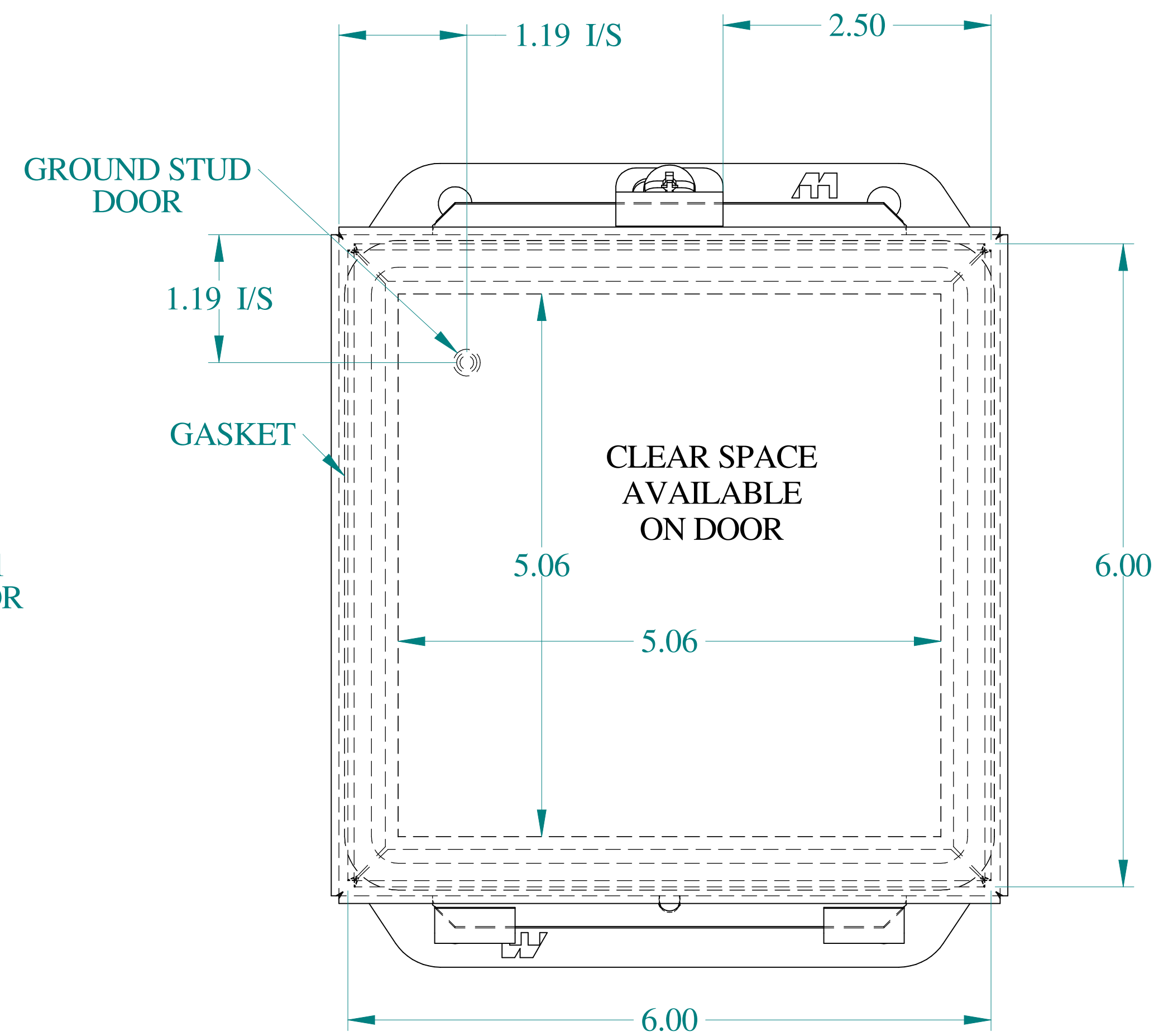
FRONT VIEW
