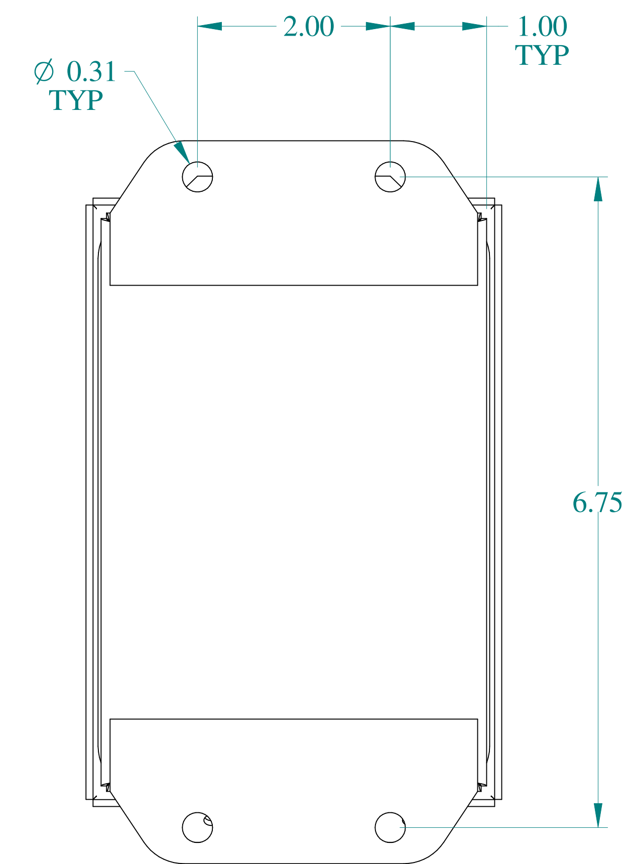
BACK VIEW
