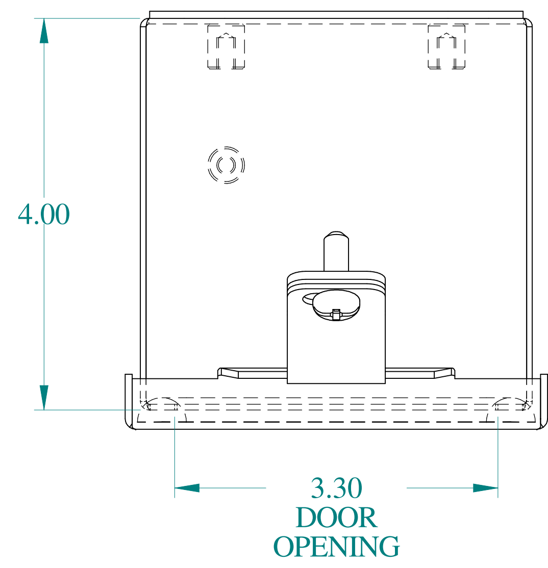
TOP VIEW
