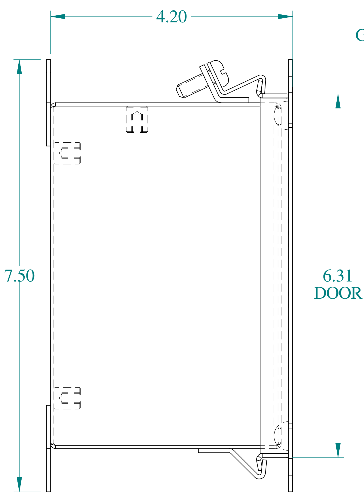
SIDE VIEW
