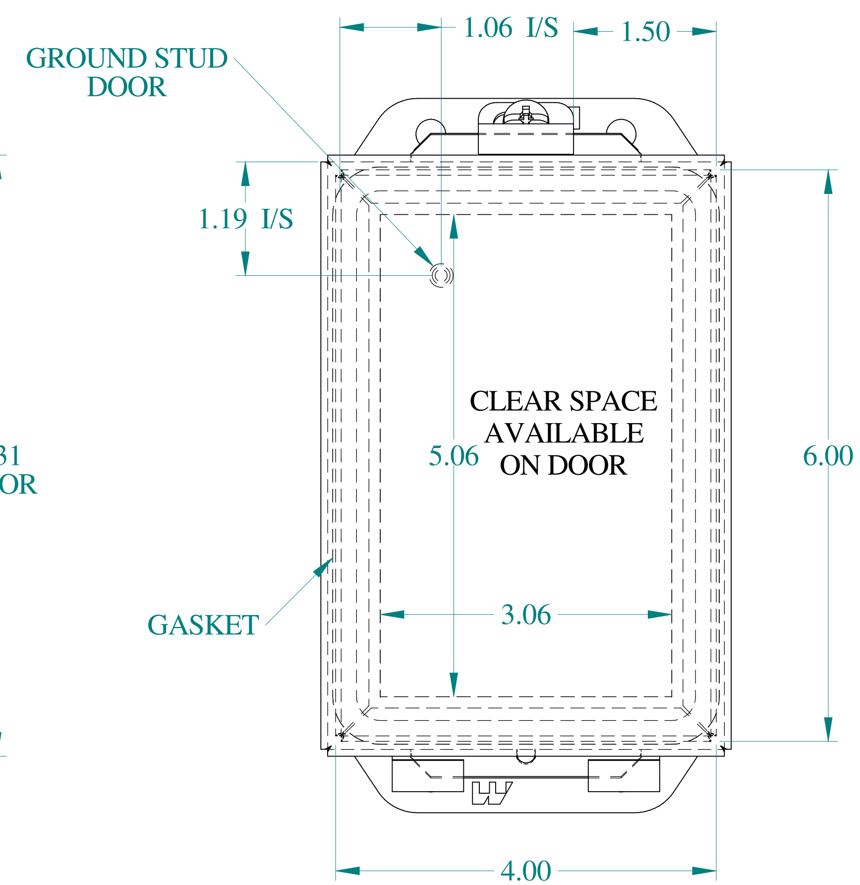
FRONT VIEW
