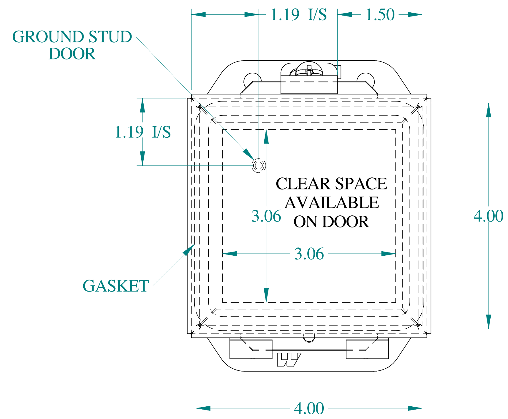
FRONT VIEW
