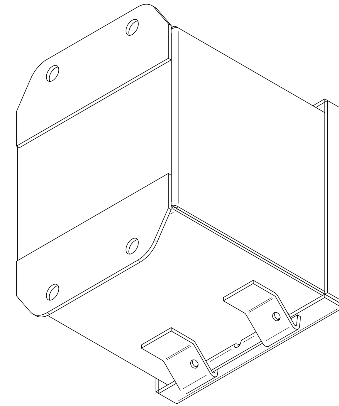
ISOMETRIC VIEWS
