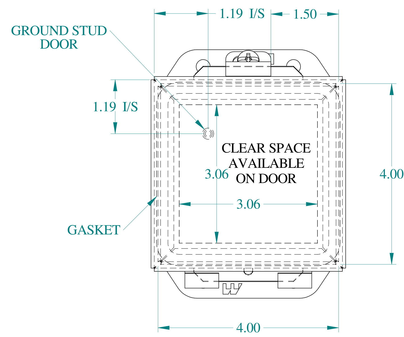
FRONT VIEW
