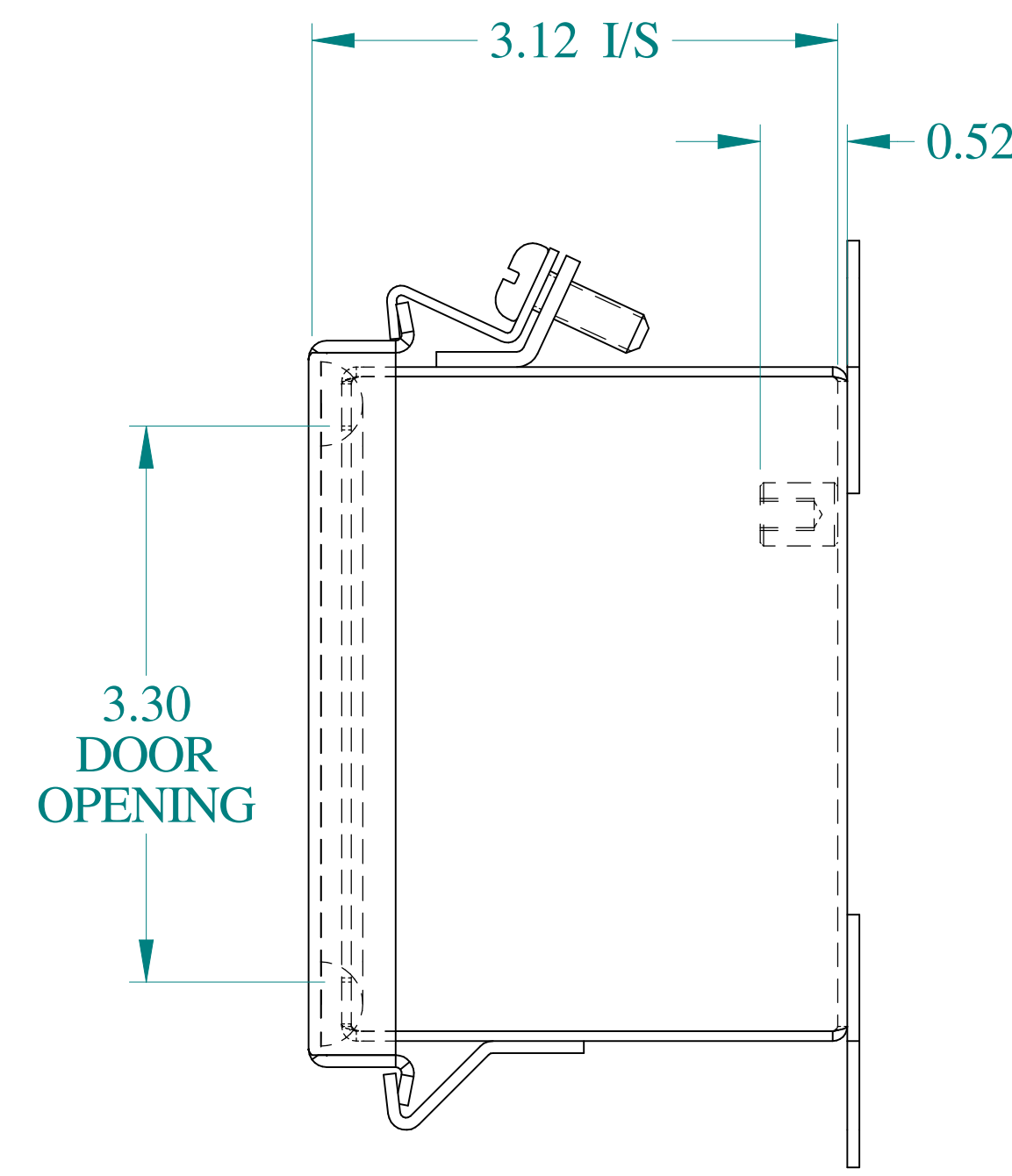
SIDE VIEW
