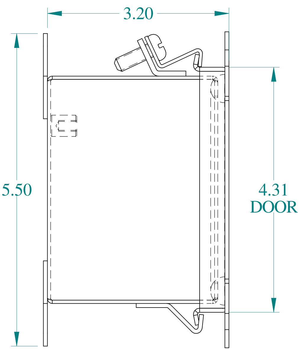
SIDE VIEW
