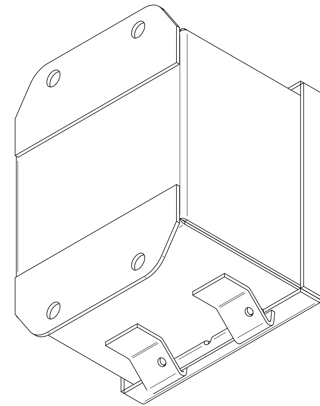
ISOMETRIC VIEWS
