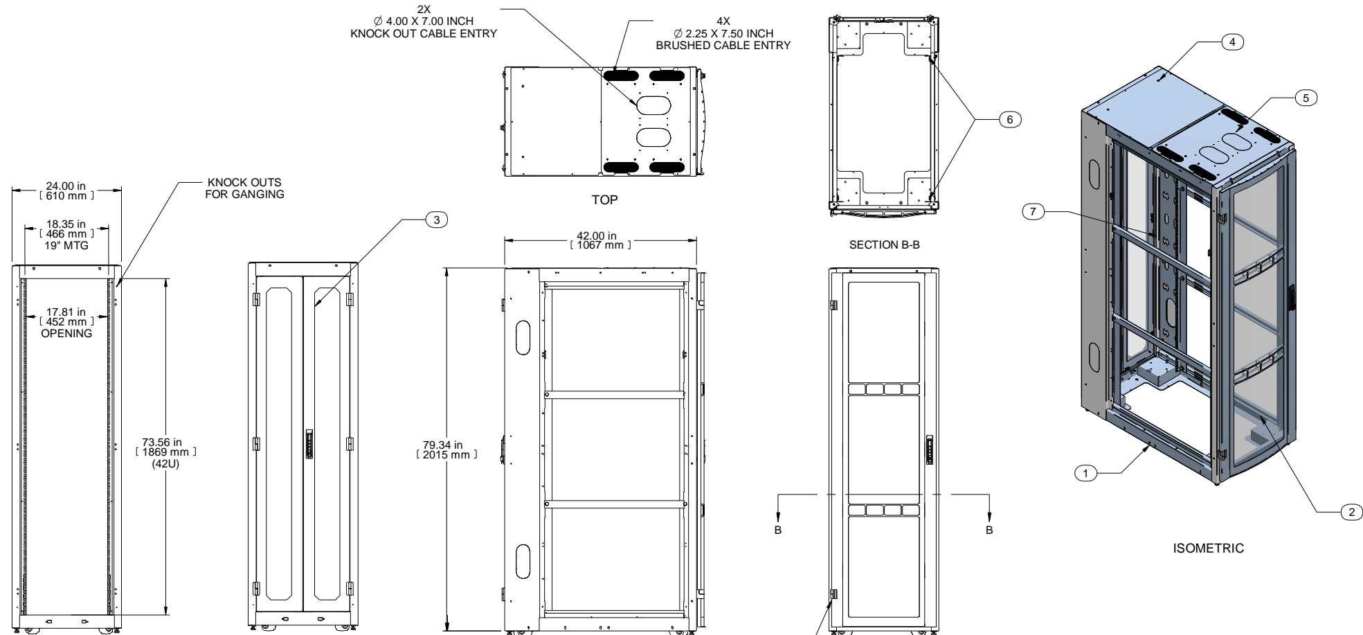
L.S. VIEW DOORS REMOVED
