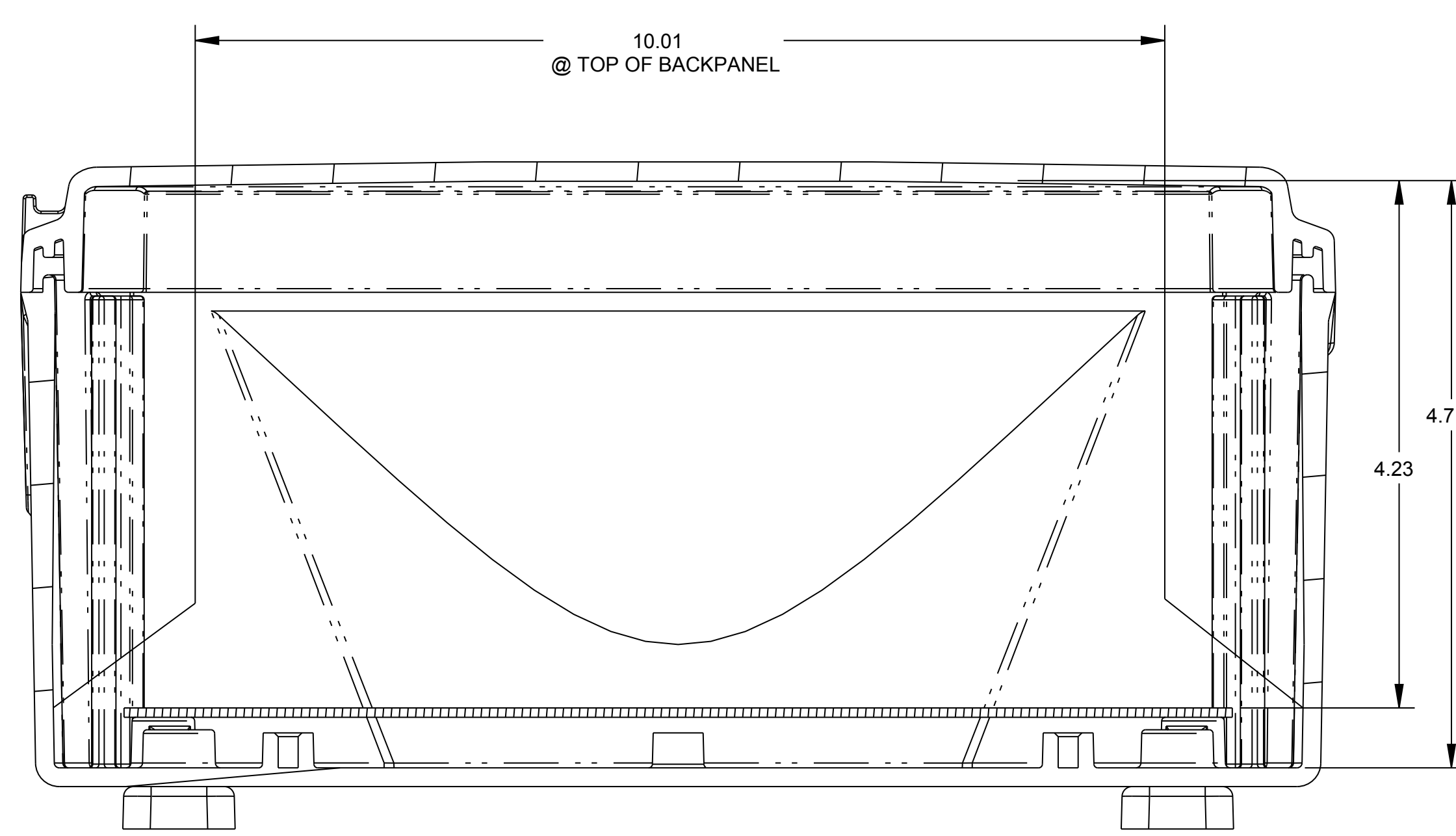
SECTION B-B
