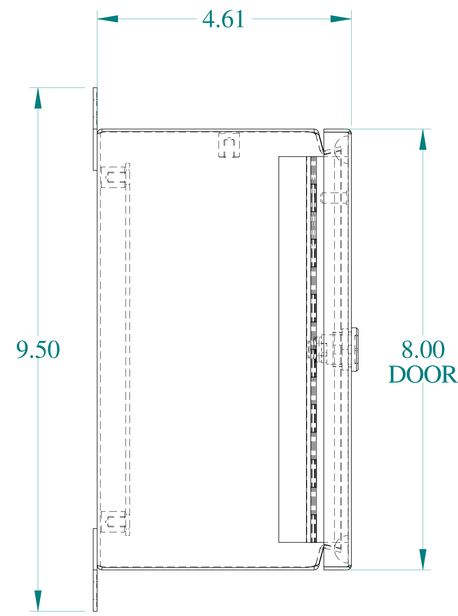
SIDE VIEW
