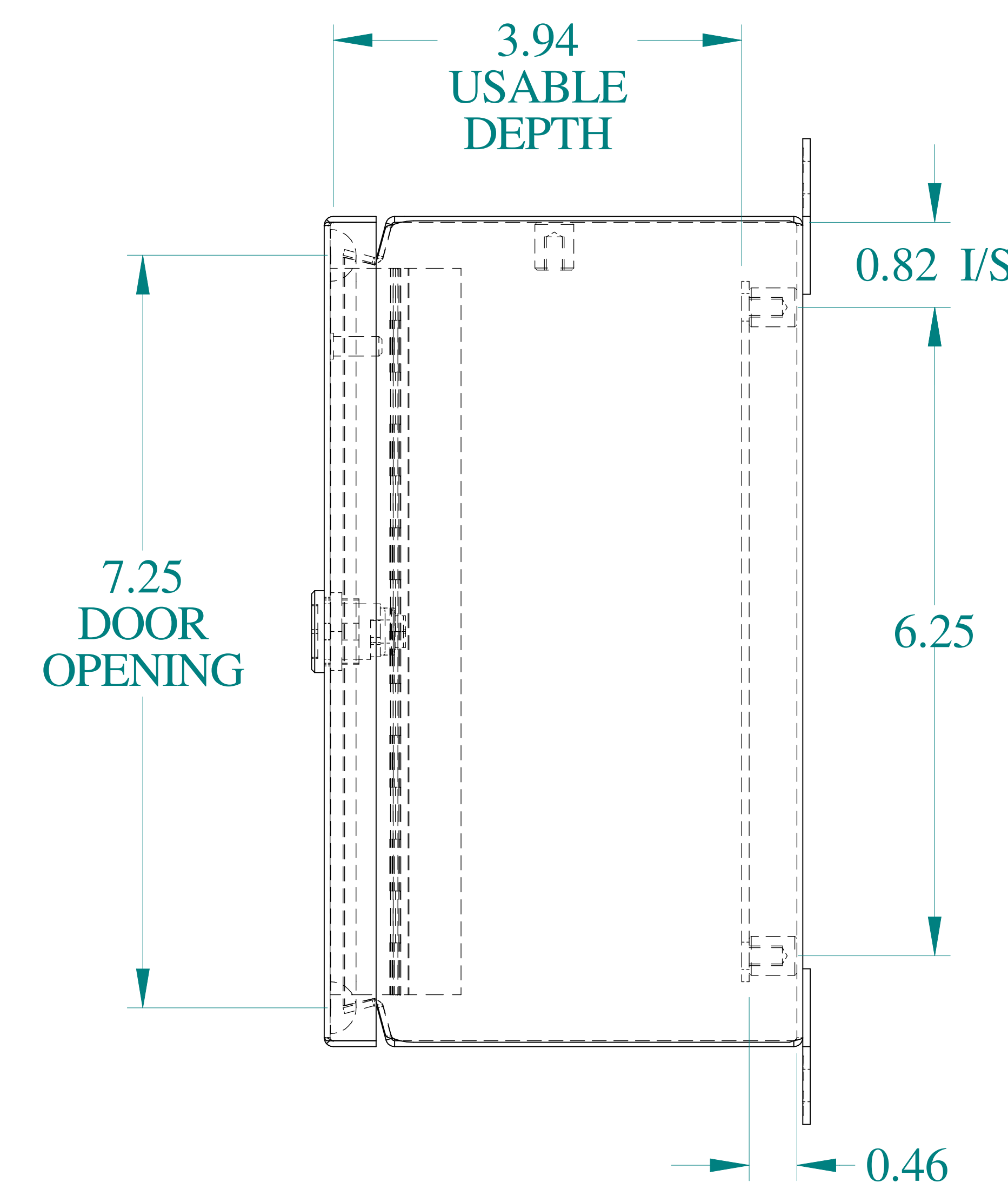
SIDE VIEW
