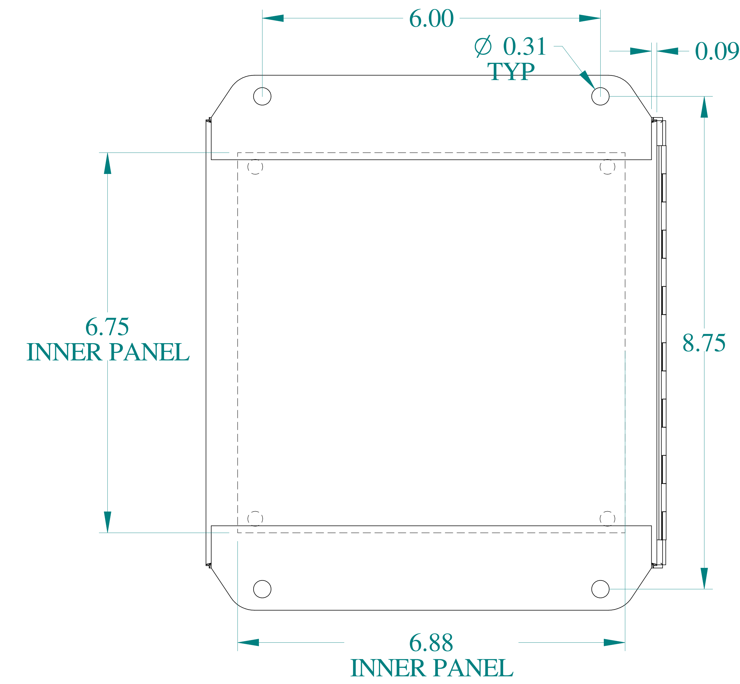
BACK VIEW
