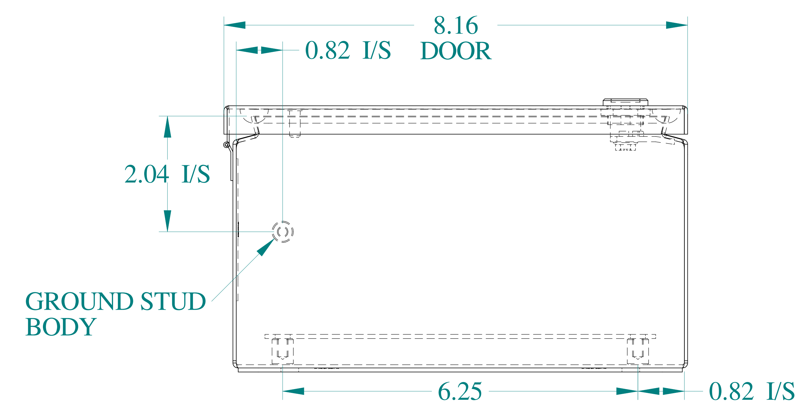
BOTTOM VIEW
