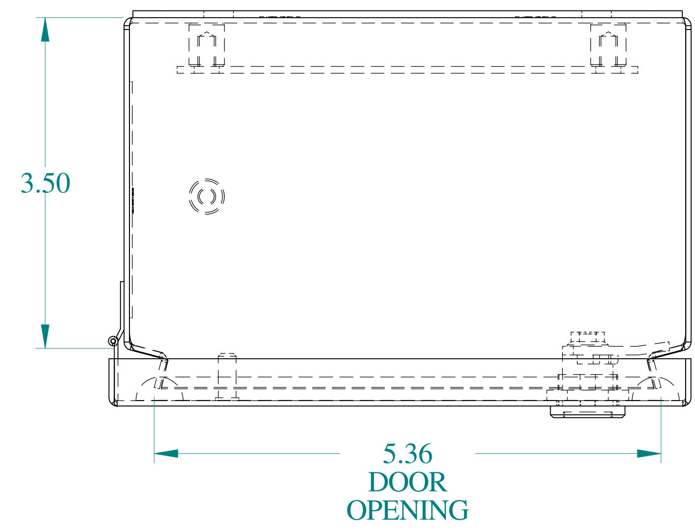
TOP VIEW
