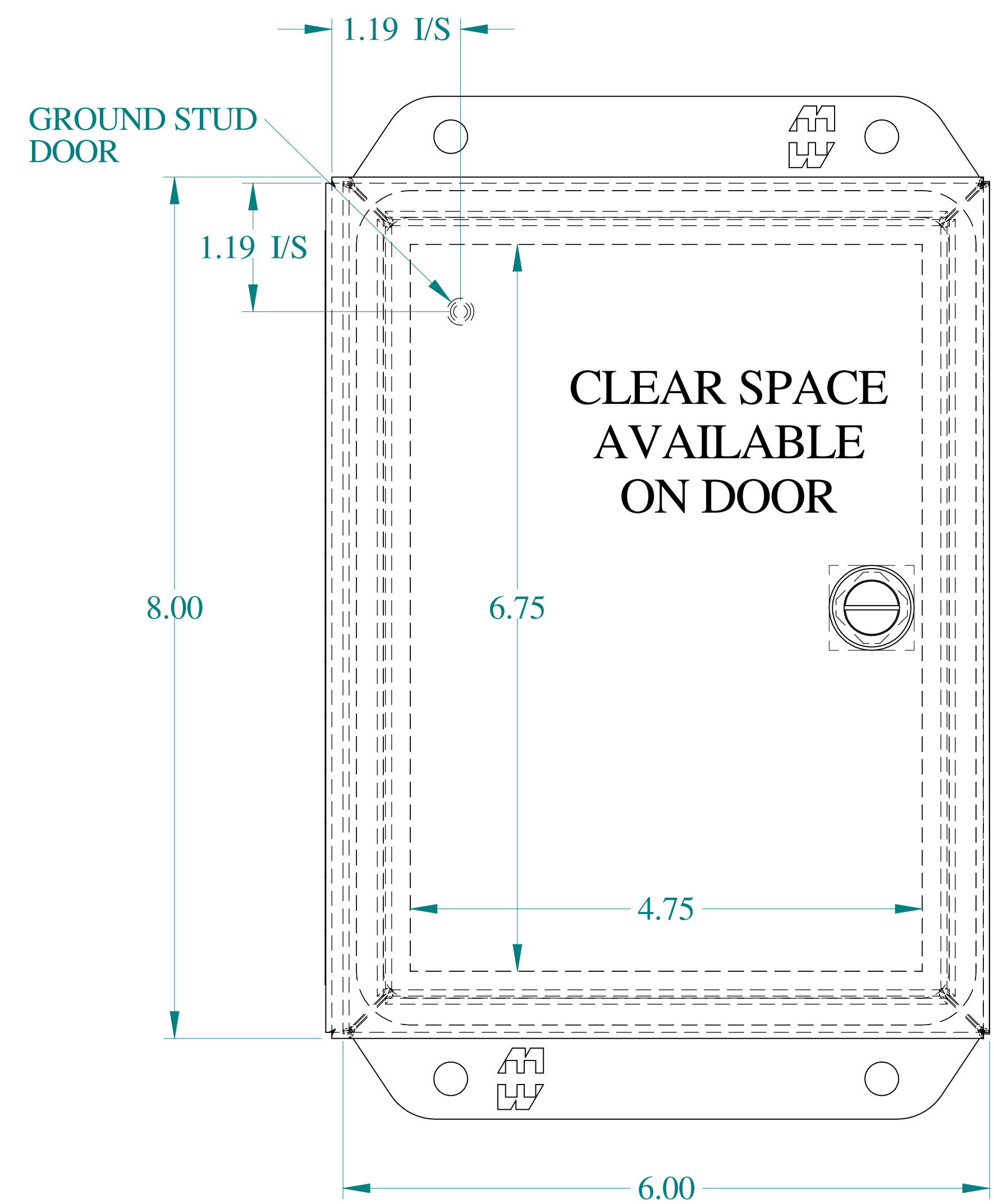
FRONT VIEW
