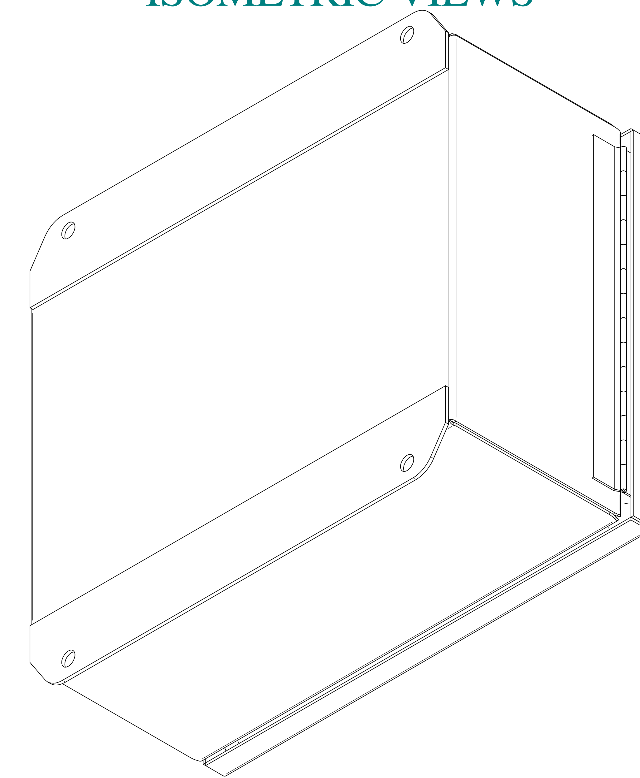
ISOMETRIC VIEWS
