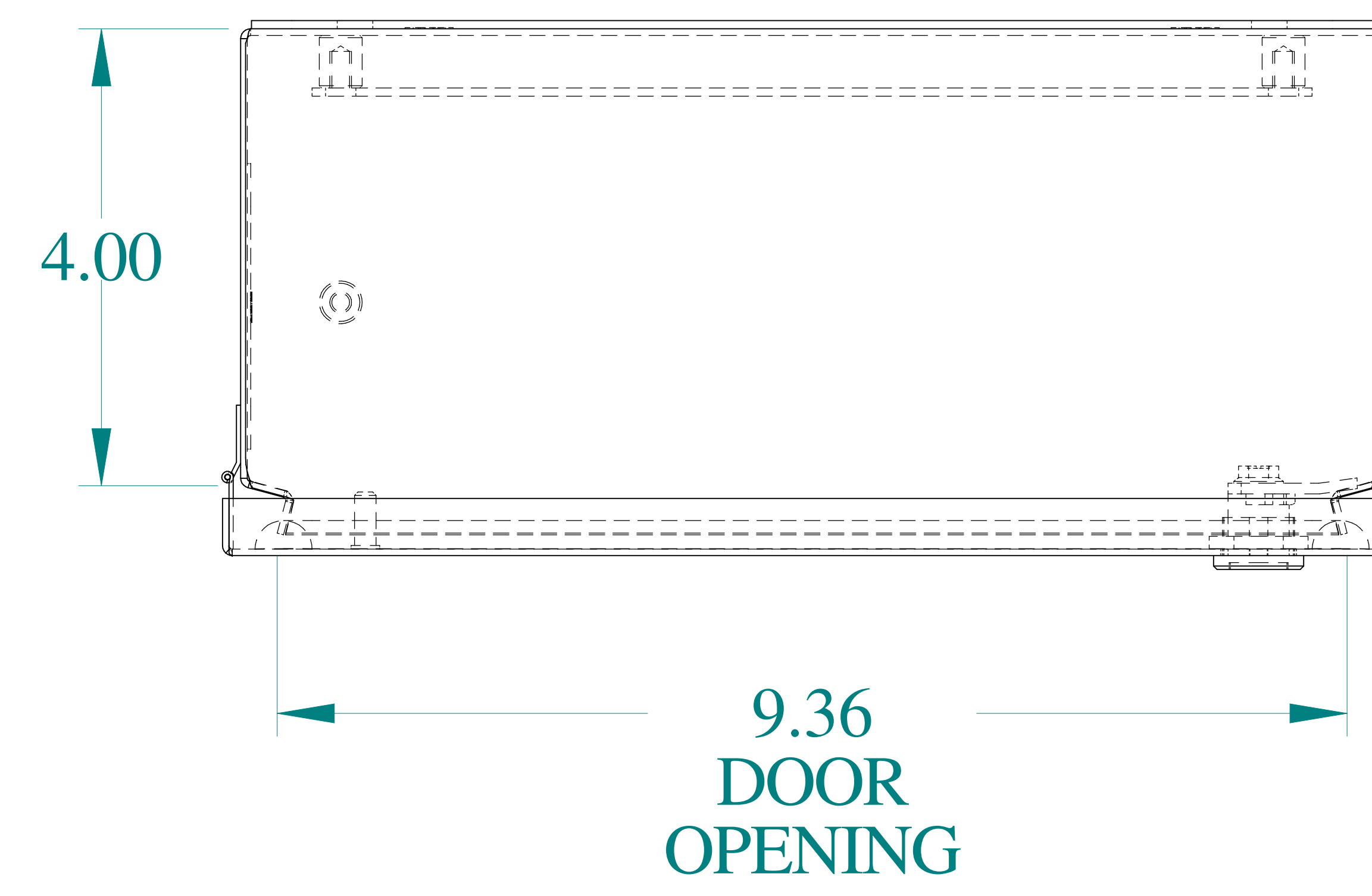
TOP VIEW
