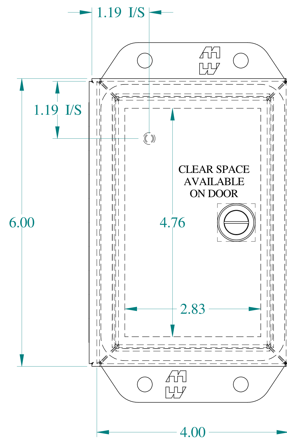
FRONT VIEW
