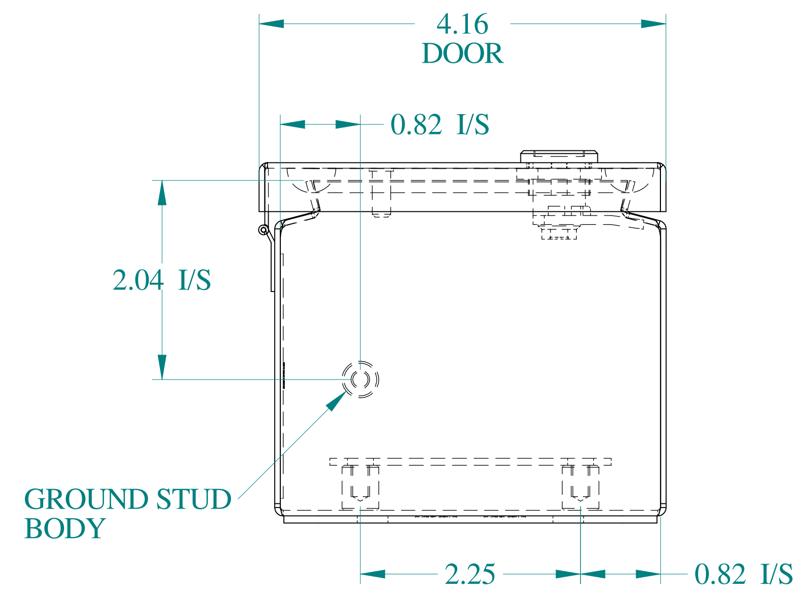
BOTTOM VIEW
