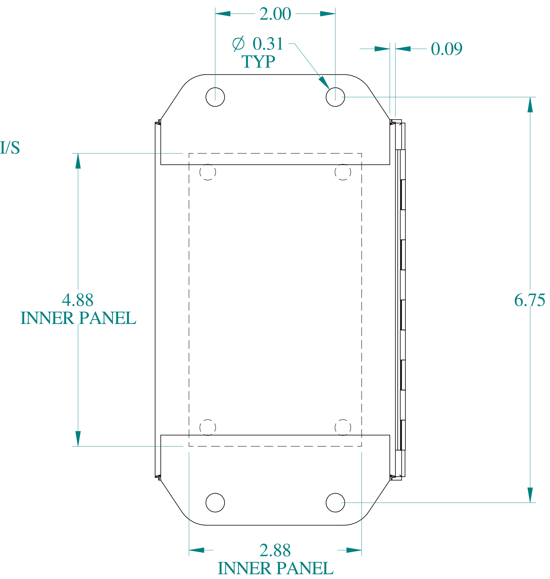
BACK VIEW
