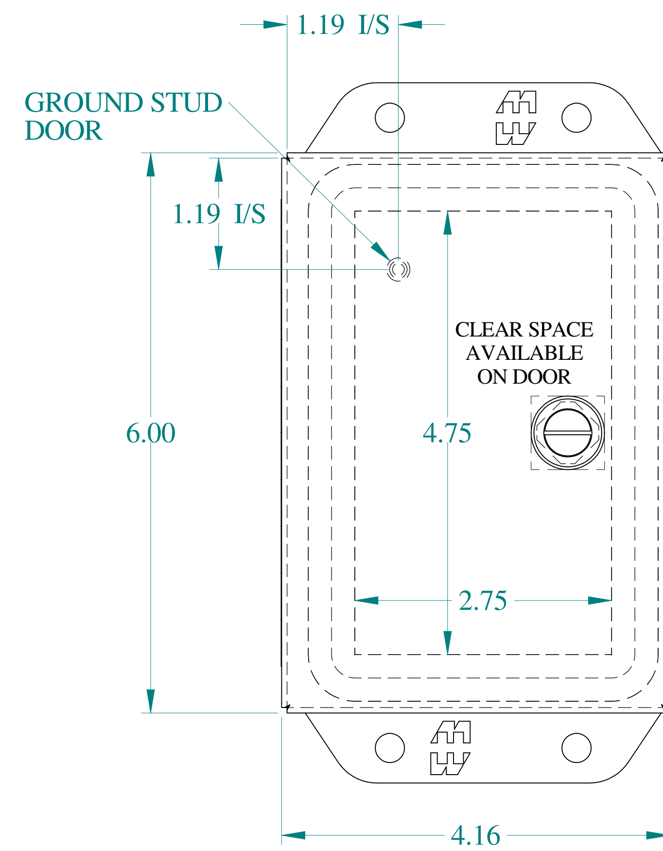
FRONT VIEW
