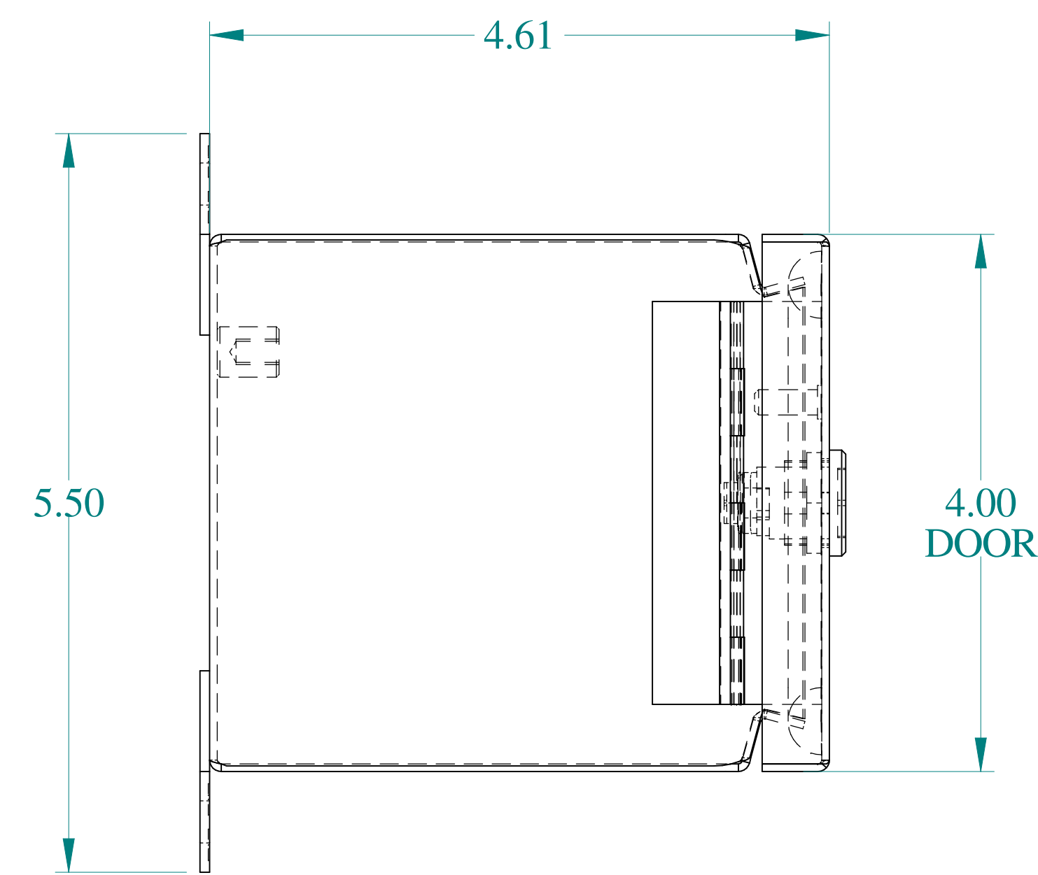
SIDE VIEW
