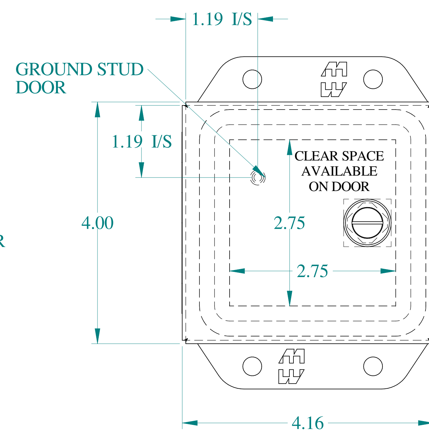
FRONT VIEW
