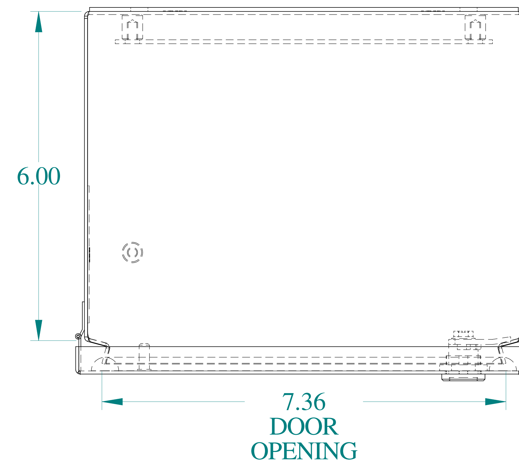
TOP VIEW
