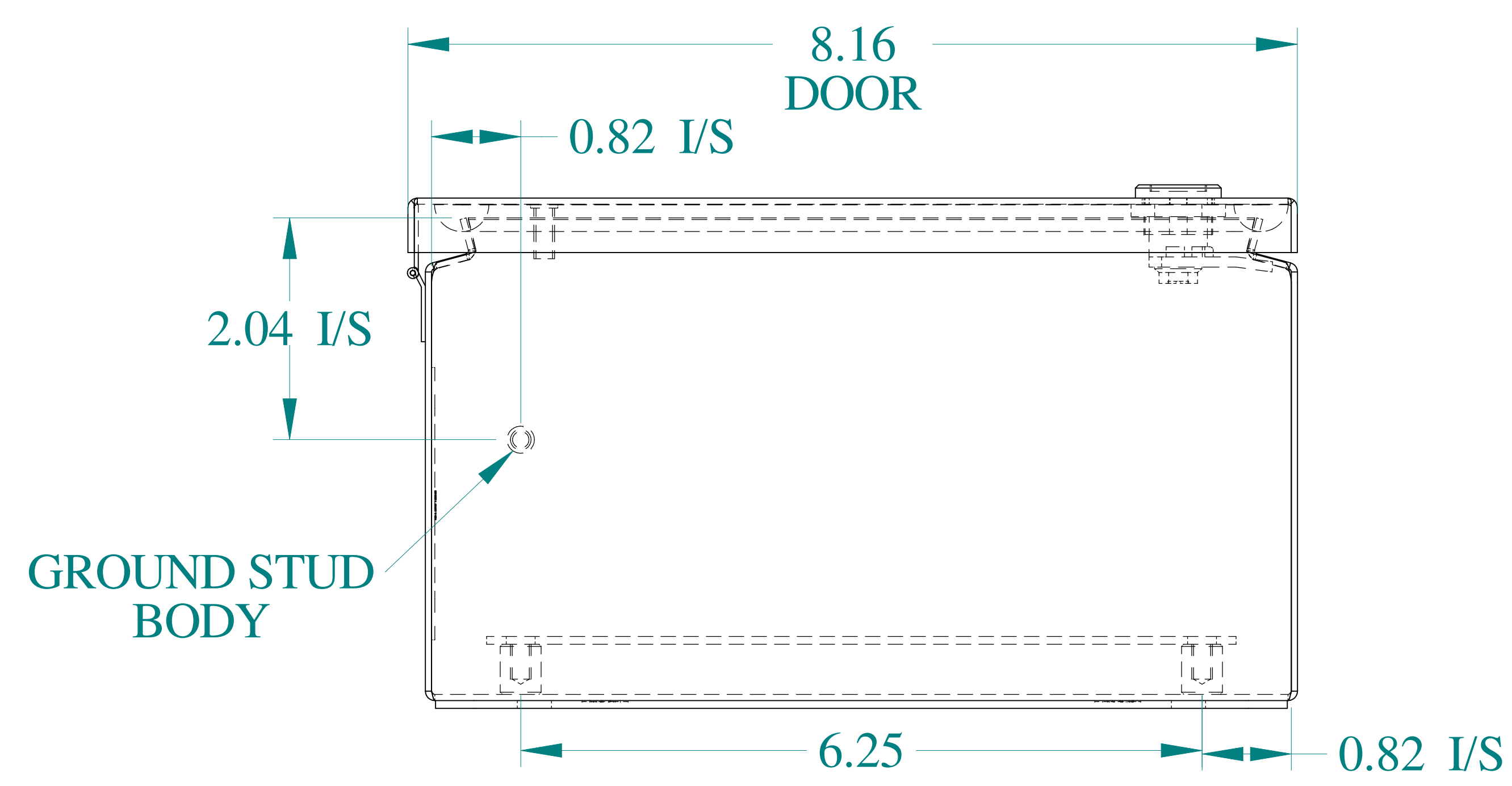
BOTTOM VIEW
