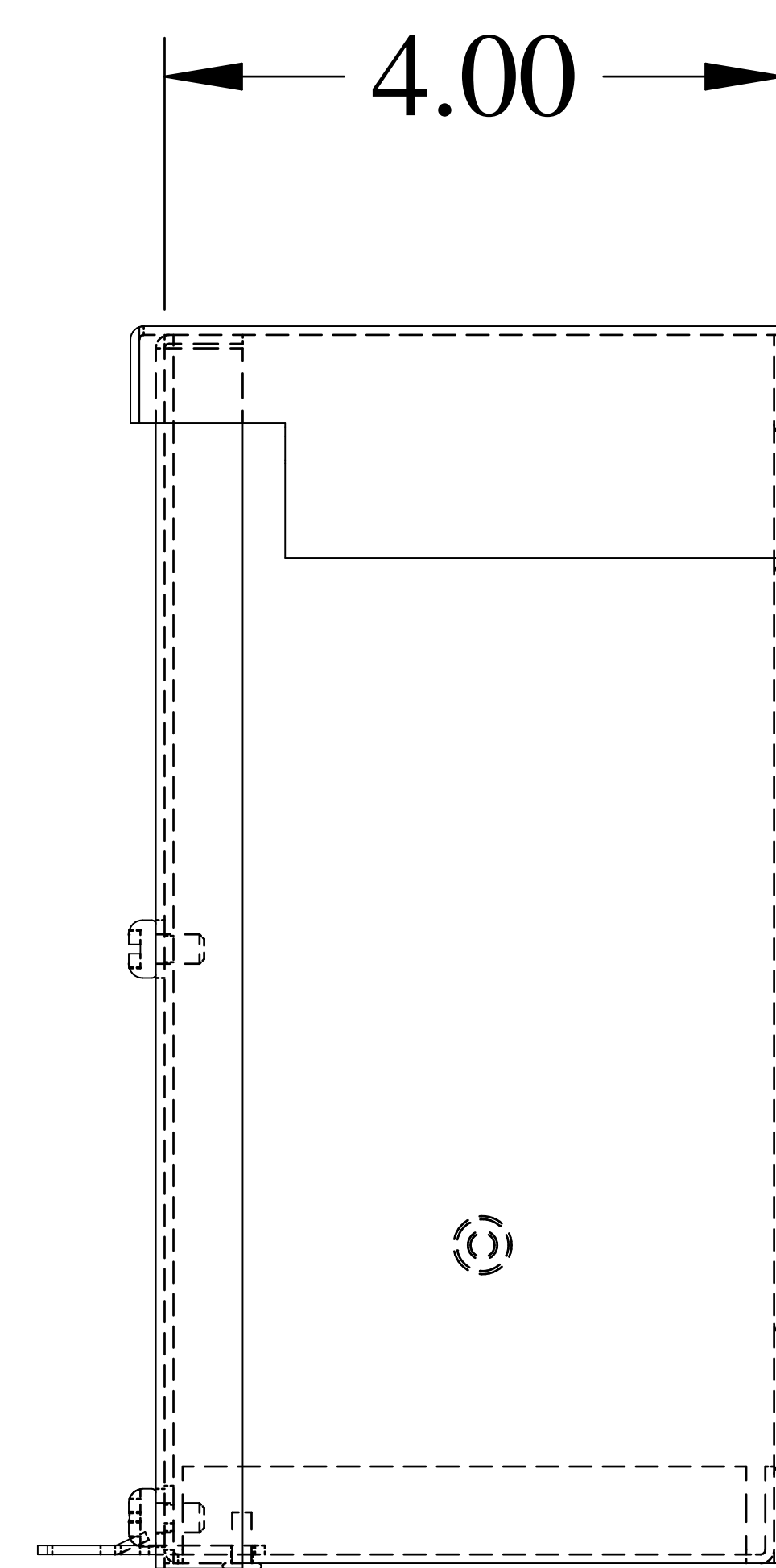
SIDE VIEW
