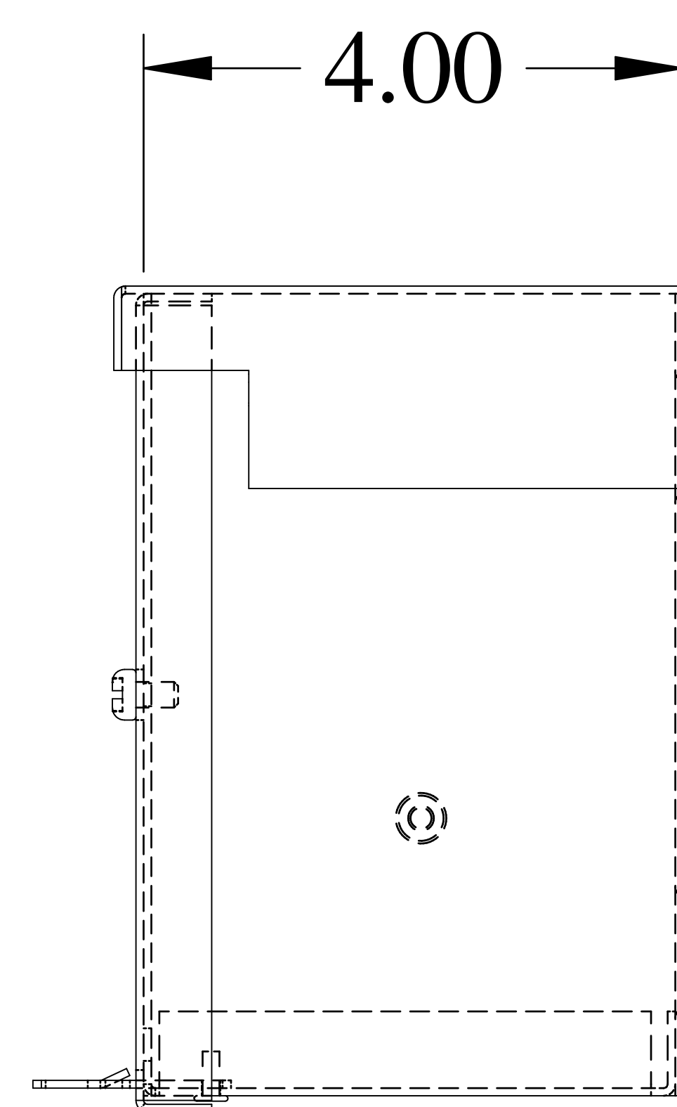
SIDE VIEW
