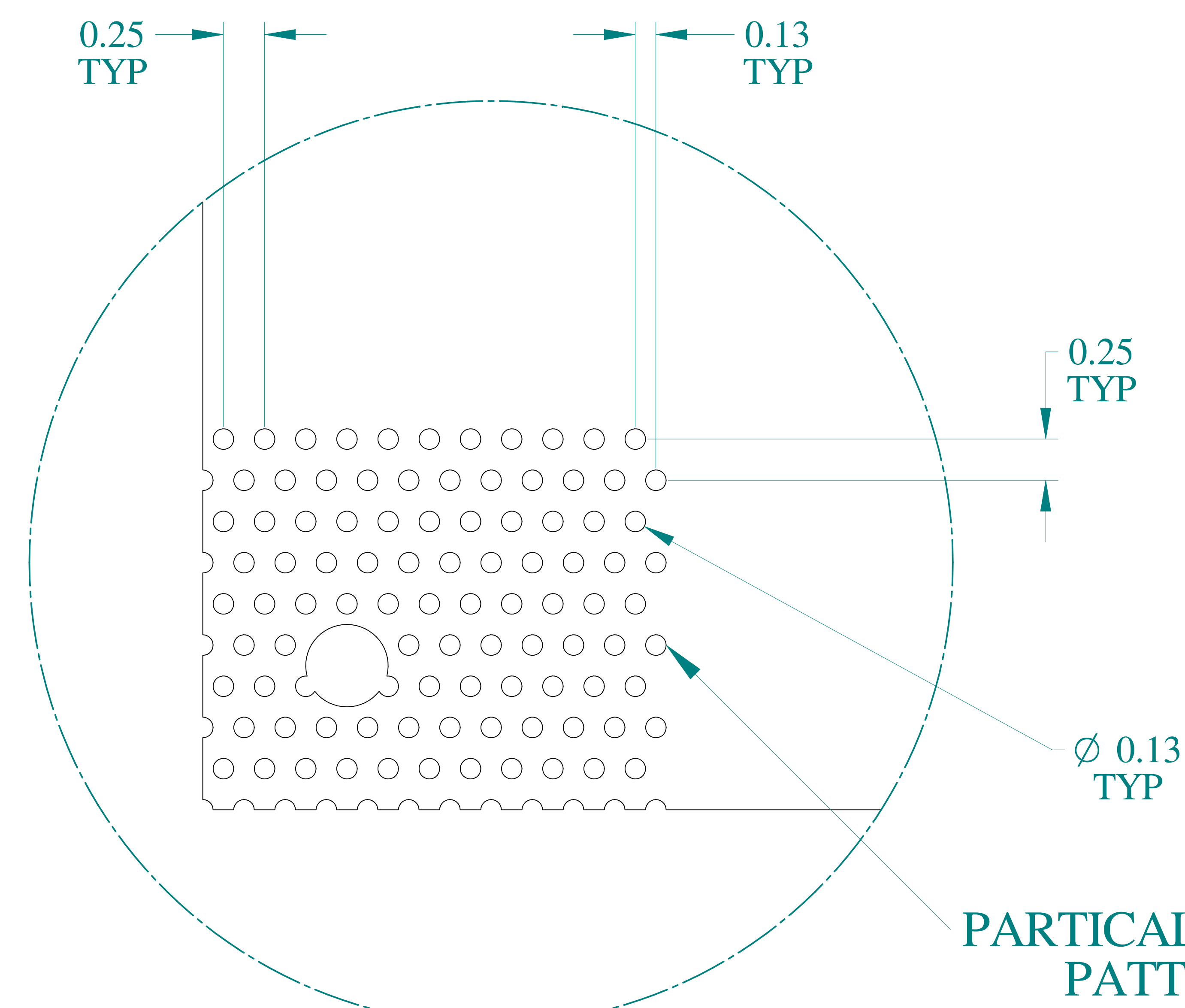
DETAIL Z
