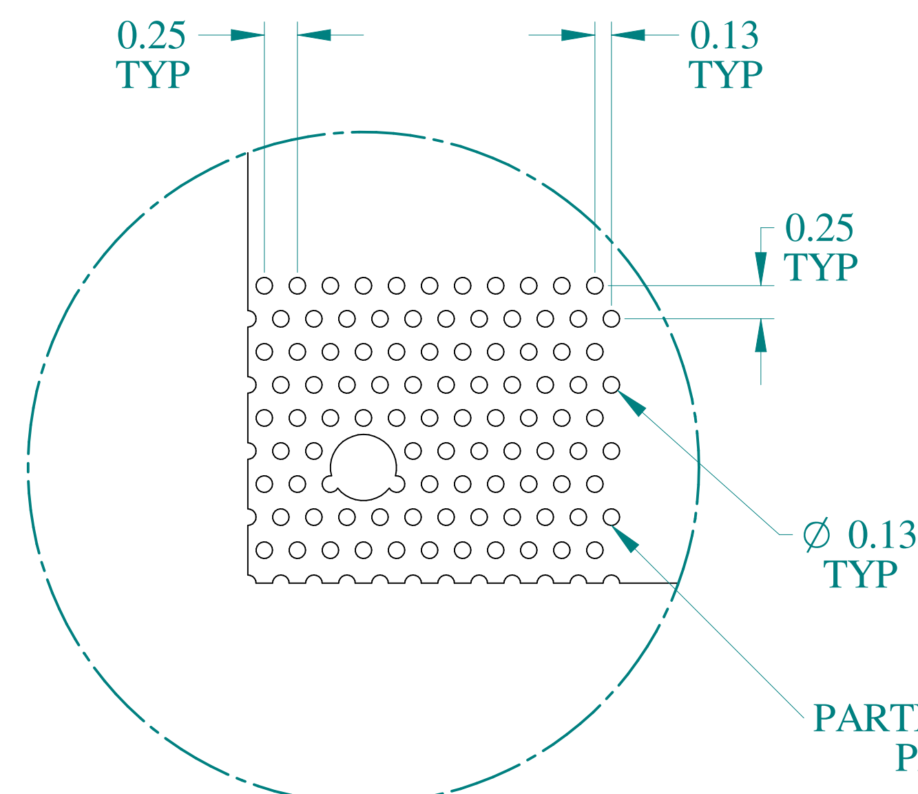
DETAIL Z
