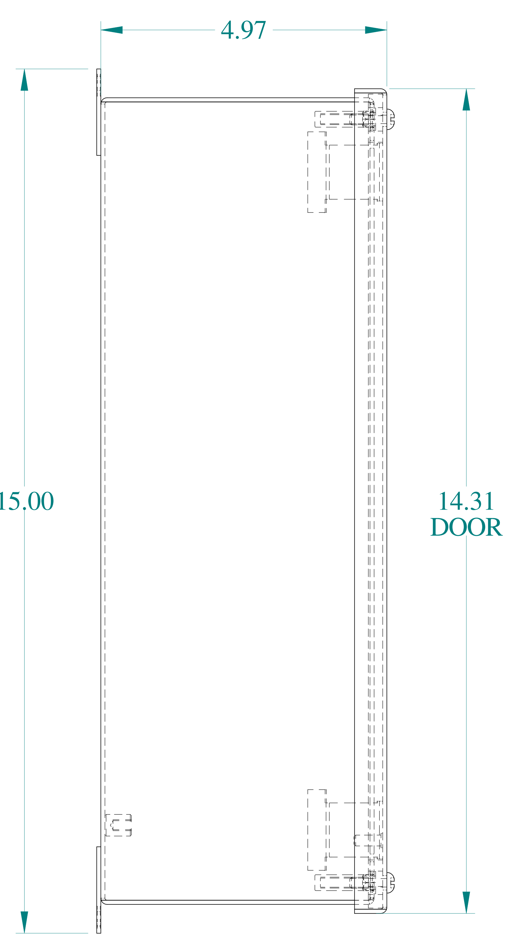
SIDE VIEW
