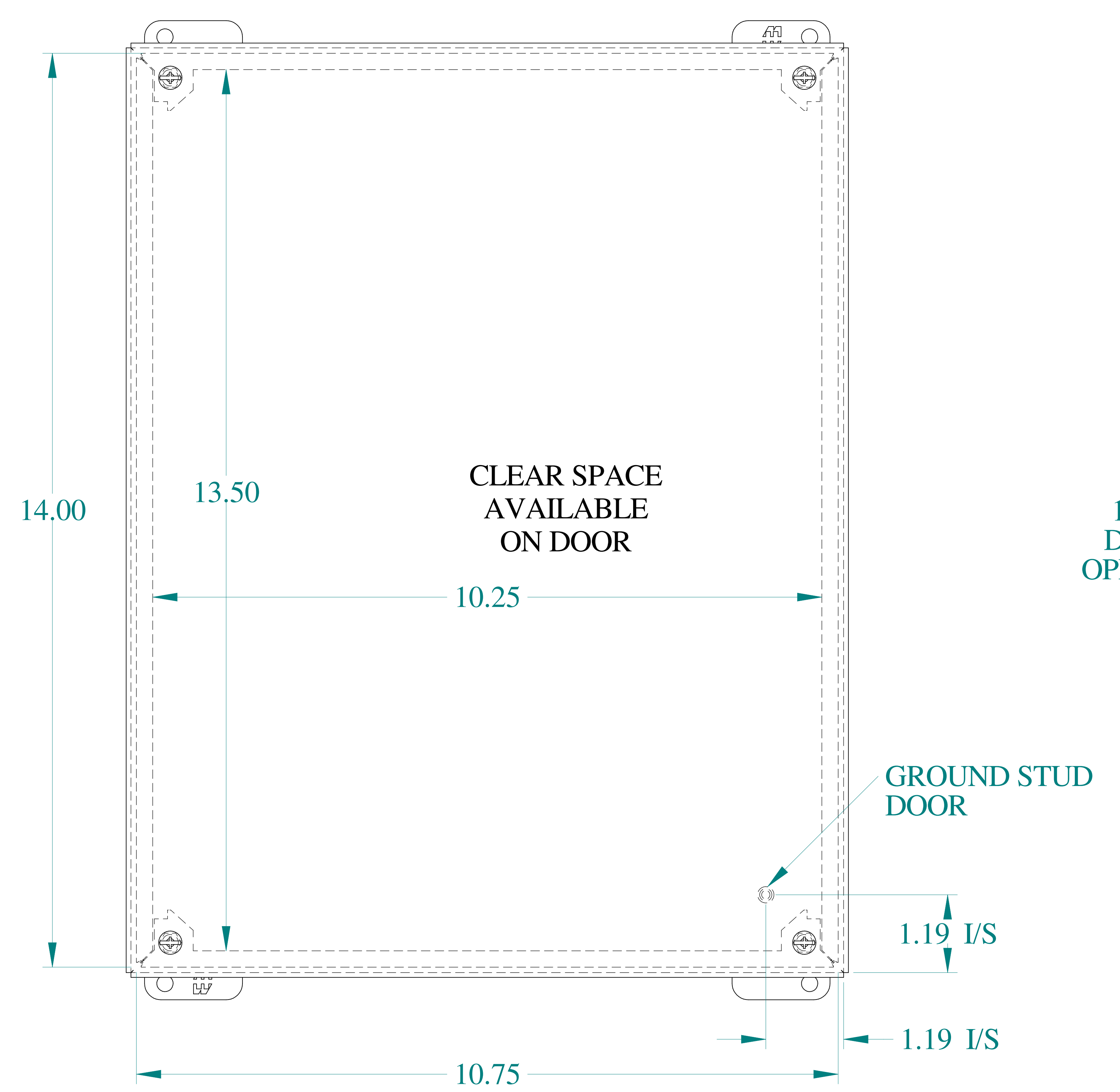
FRONT VIEW
