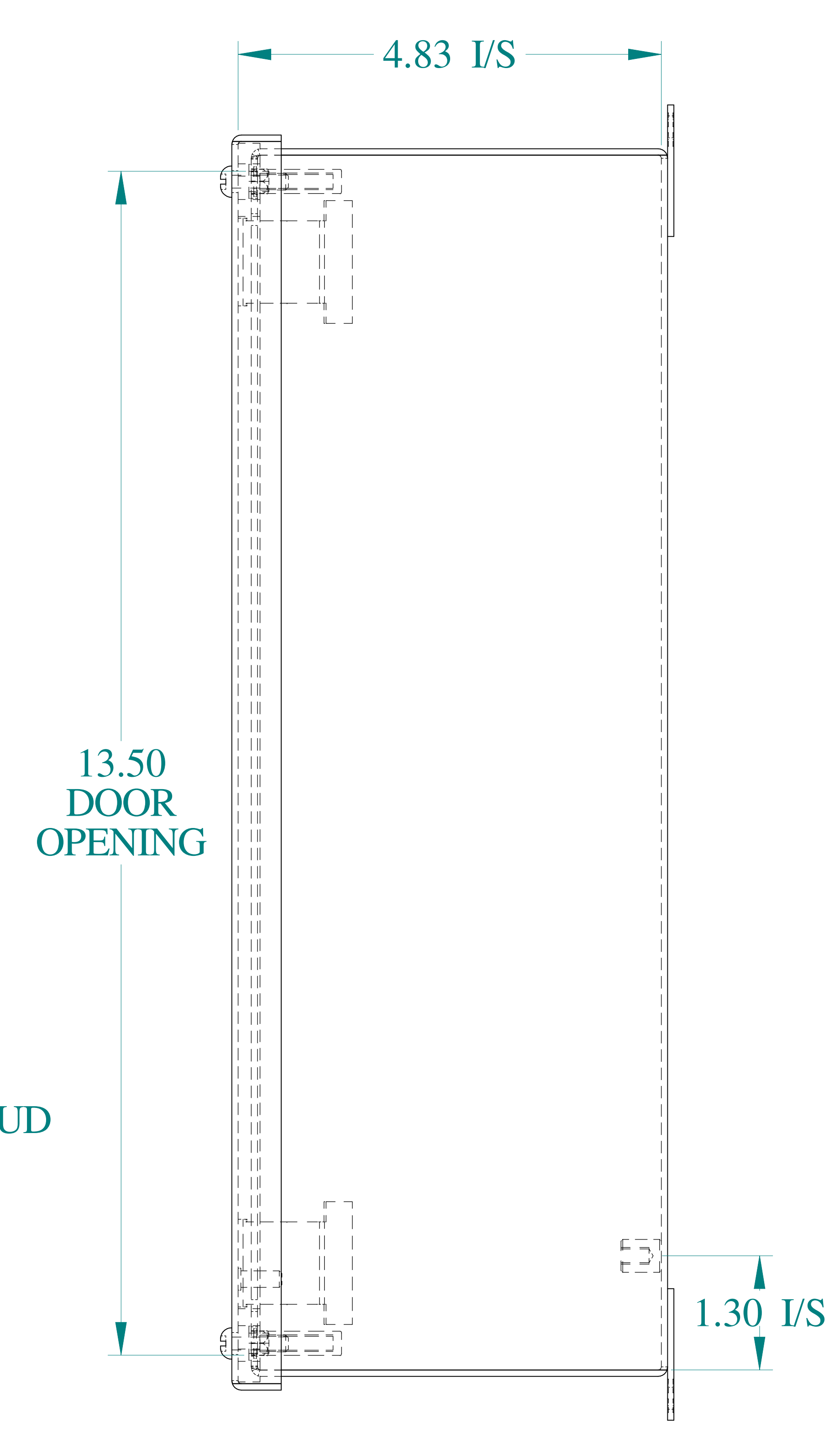
SIDE VIEW
